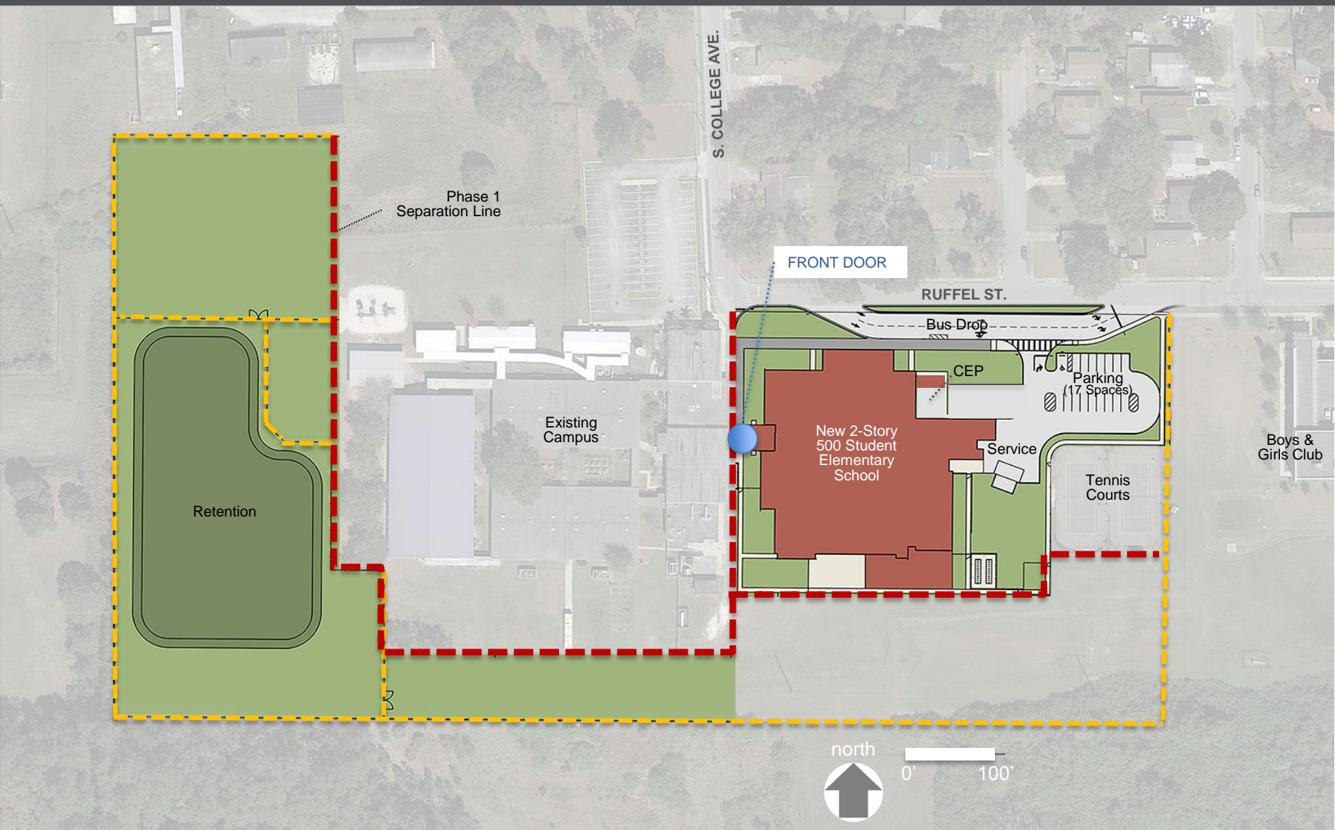
Site Plan – PHASE 1 – New School, play amenities, service, staff parking, and retention pond
